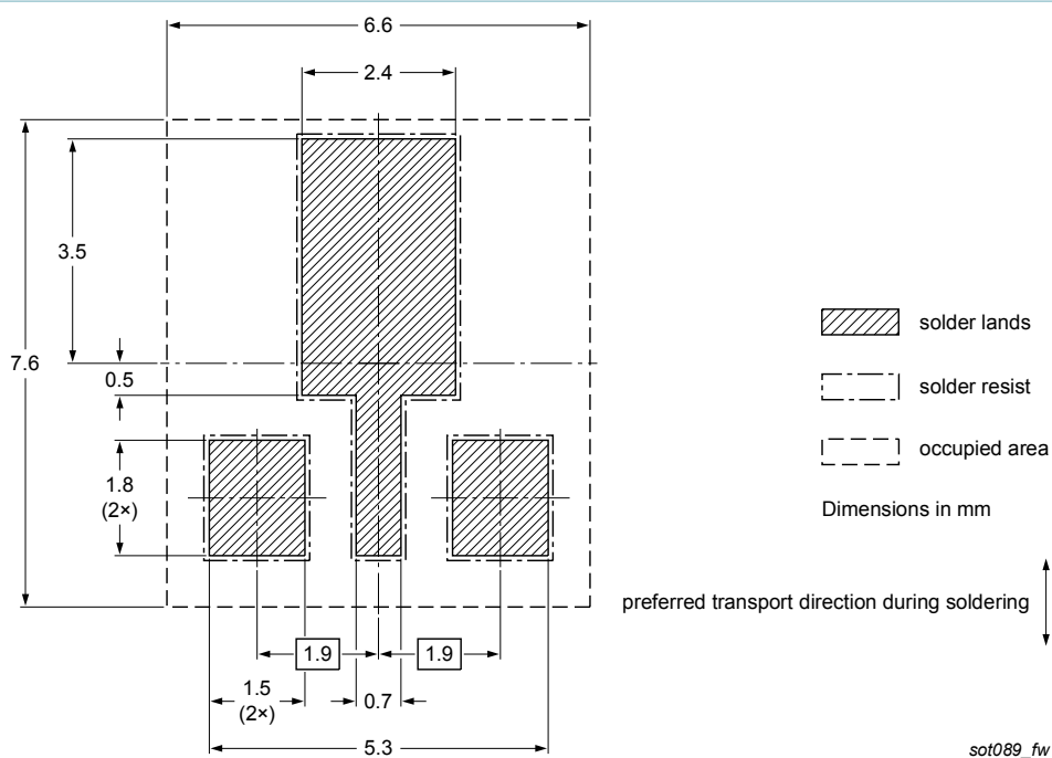
Fig. 13. Wave soldering footprint for SOT89
