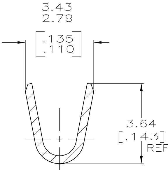
SECTION X-X SCALE 10:1
