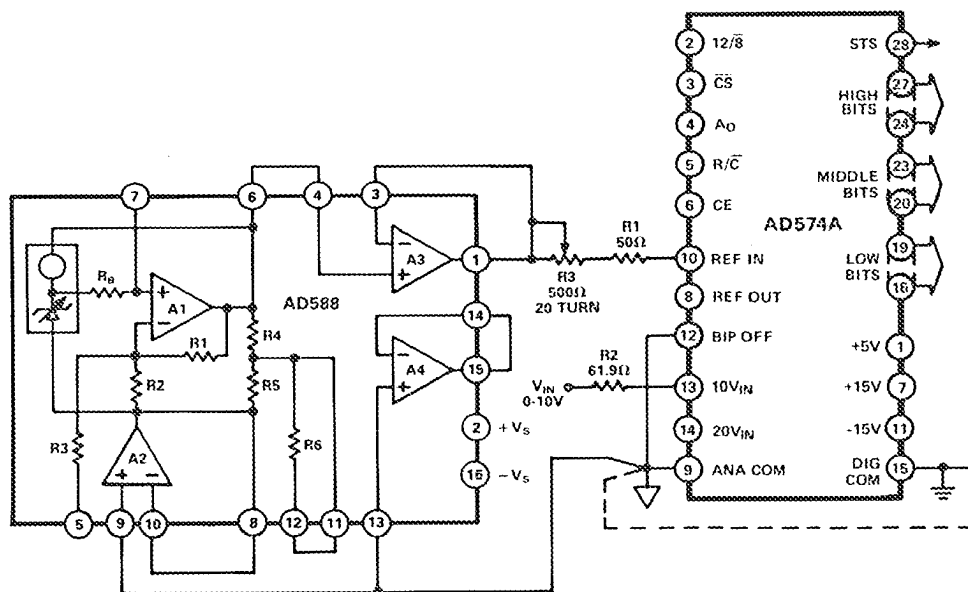
Figure 17. AD588/AD574A Connections
