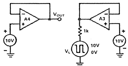
Figure 13a. Load Crosstalk Test Circuit
