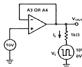
Figure 10a. Transient Load Test Circuit
