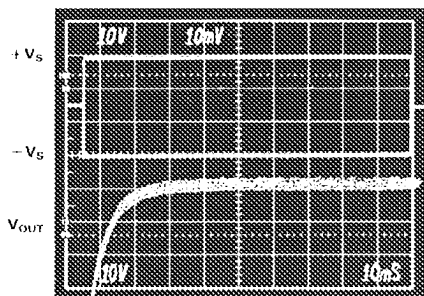
Figure 6. Turn-On with 1 \mu\text{F} C_N
