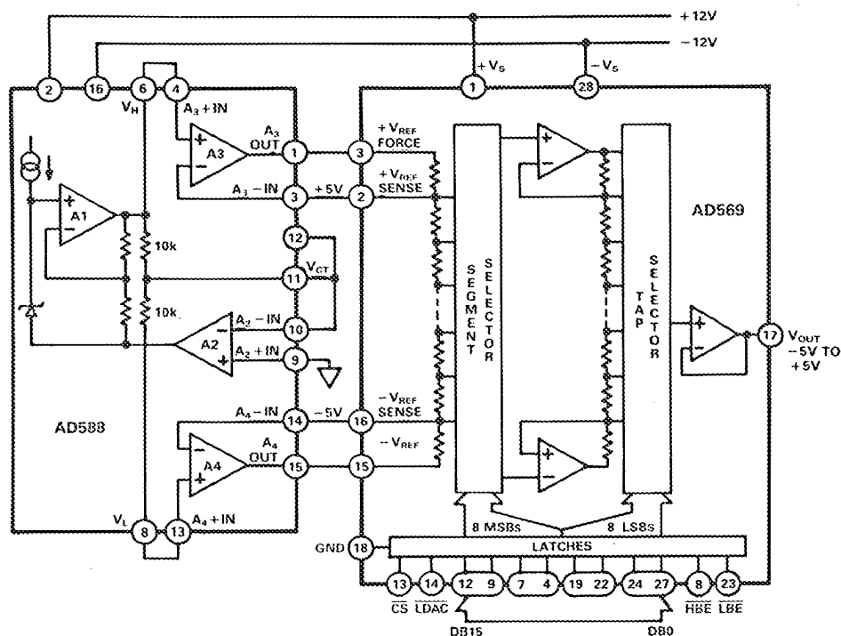
Figure 16. High Accuracy \pm 5 V Tracking Reference for AD569
