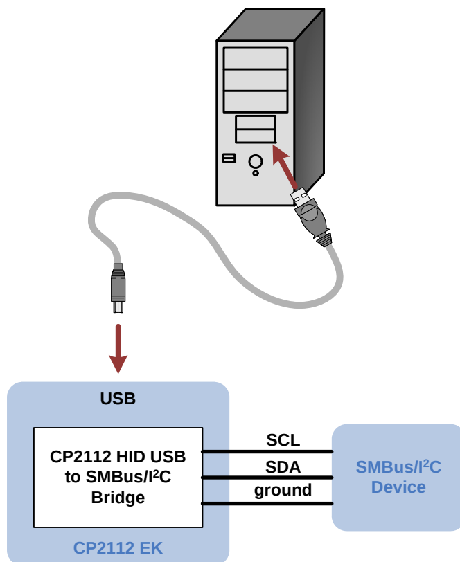
Figure 1. Hardware Setup
