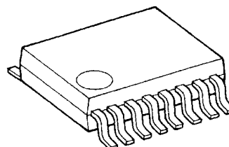
SSOP16-P-225-0.65B
