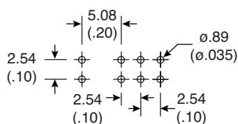
P.C. Mounting
