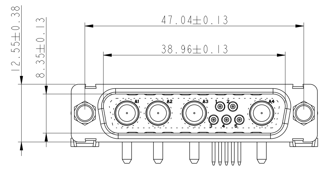
LAYOUT AND CONNECTOR DIMENSIONS For PCB hole diameters see table I sheet I
