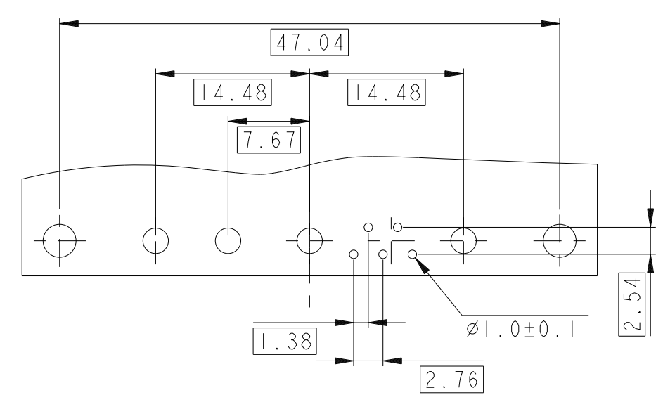
LAYOUT AND CONNECTOR DIMENSIONS For PCB hole diameters see table I sheet I
