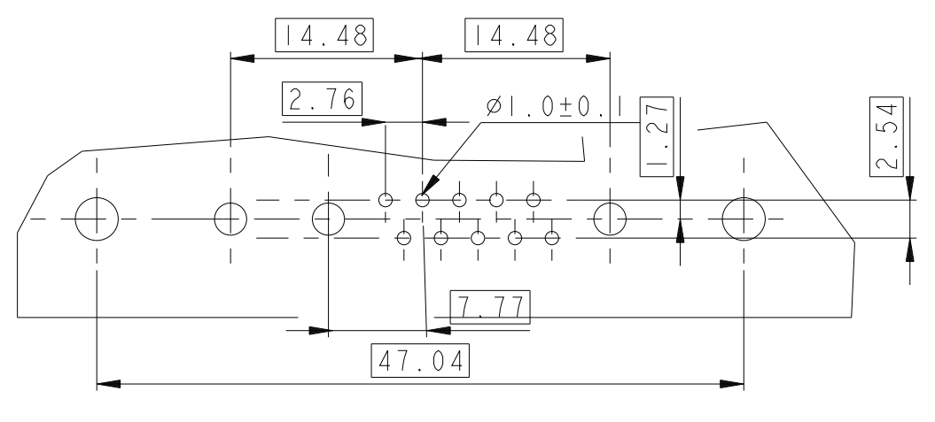
LAYOUT AND CONNECTOR DIMENSIONS For PCB hole diameters see table I sheet I
