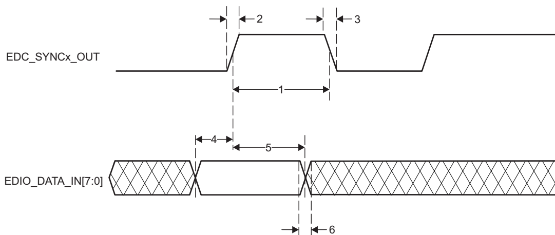
Figure 7-103. PRU-ICSS ECAT Input Validated With SYNCx Timing
