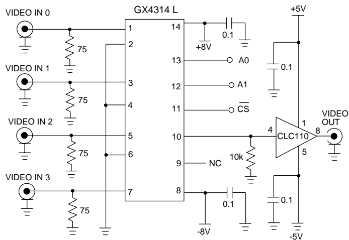
Fig. 6 Test Circuit
