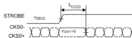
FIGURE 20. Serializer Clock Propagation Delay
