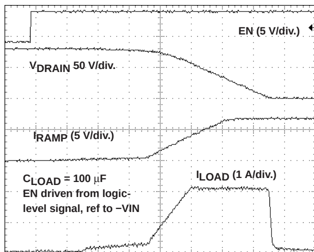
START-UP FROM ENABLE ASSERTION
