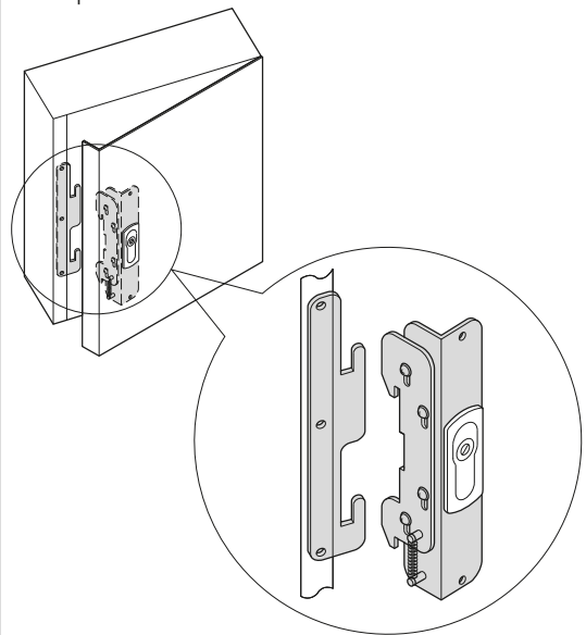
取付け例 Example of installation
