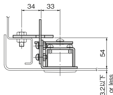
取付け例 Example of installation
