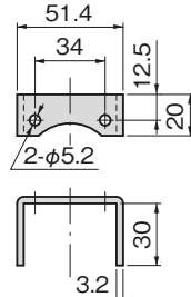
取付け金具 Installation plate
