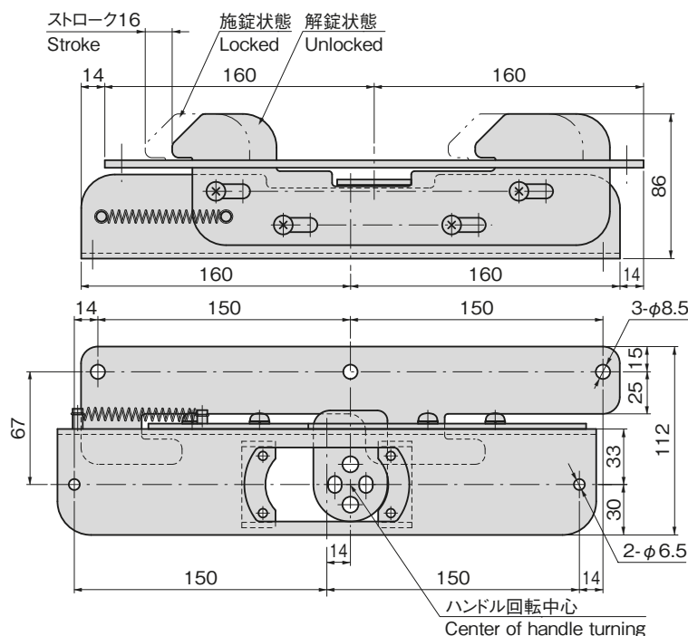
止め金 Stopper plate
