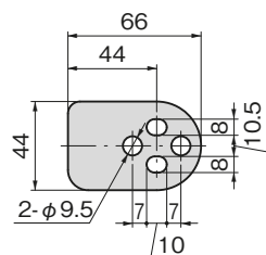
止め金 Stopper plate
