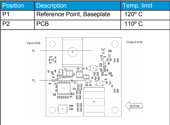
Base plate
