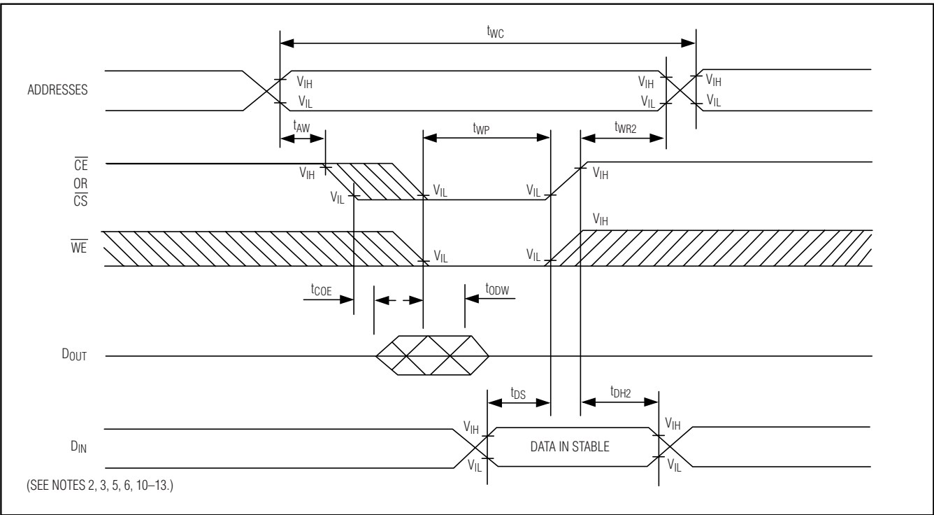
Write Cycle 2
