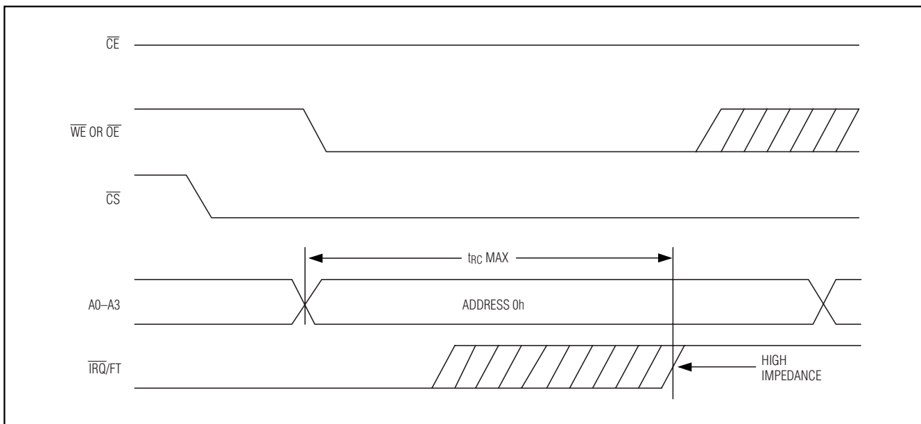
Figure 1. Clearing Active IRQ Waveforms
