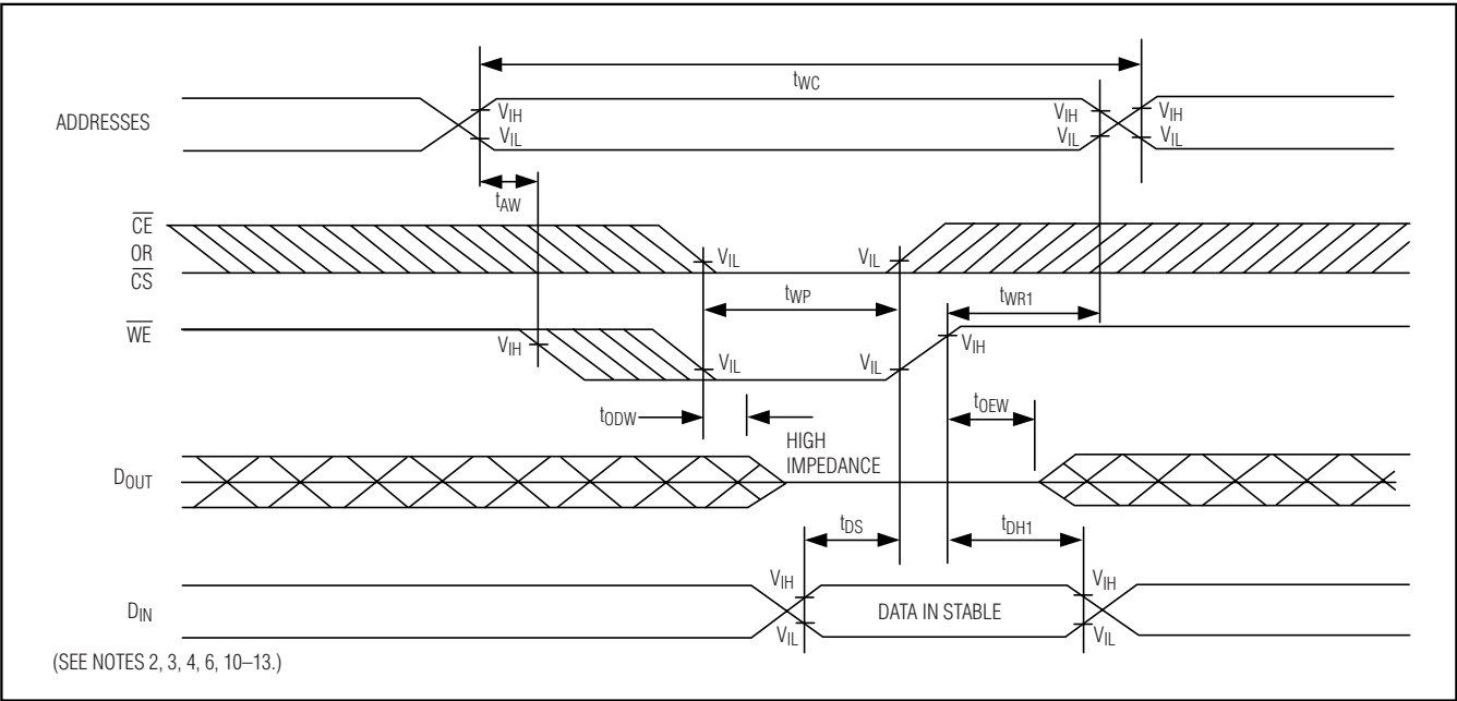
Write Cycle 1
