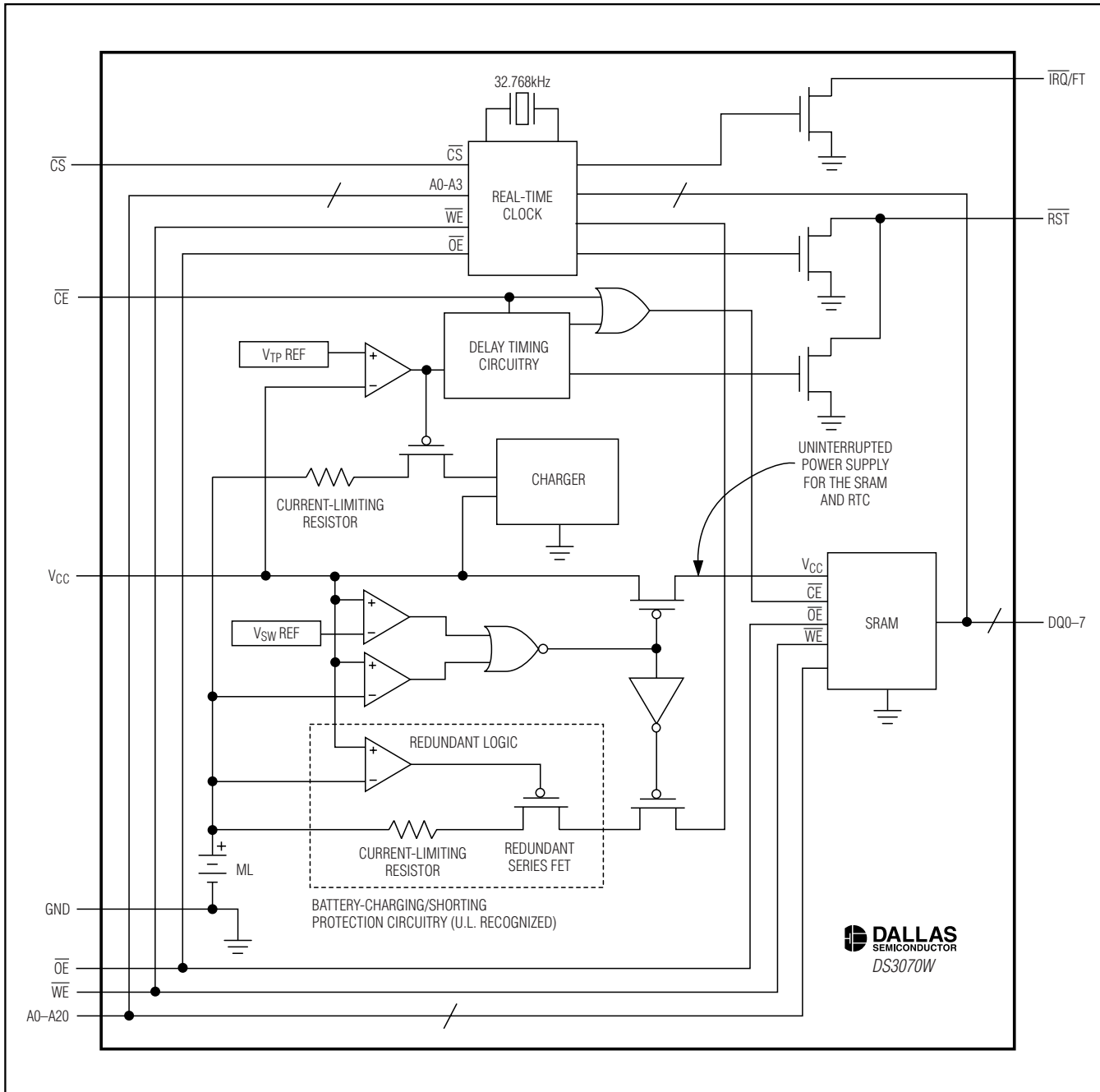
Functional Diagram
