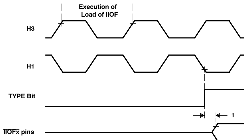
Figure 19. Change of \overline{\text{IIOF}}_{\text{x}} From Input to Output Mode
