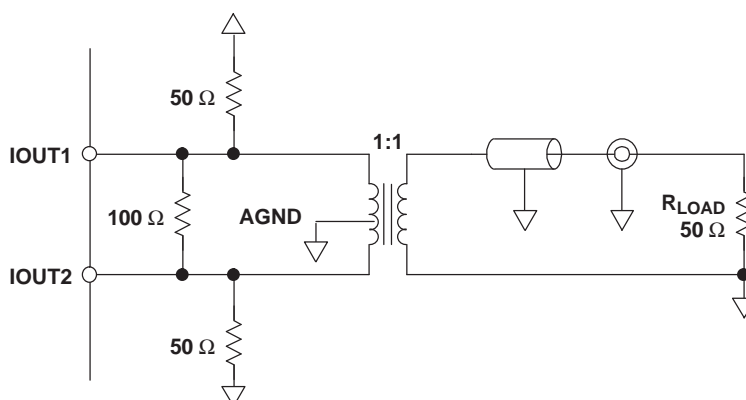
Figure 22. Driving a Doubly-Terminated 50- \Omega Cable Using a 1:1 Impedance Ratio Transformer
