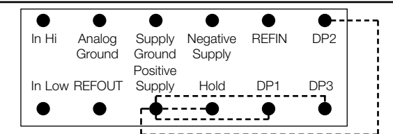
Optional Connections
