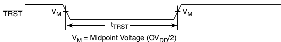
Figure 9. \overline{\text{TRST}} Timing Diagram
