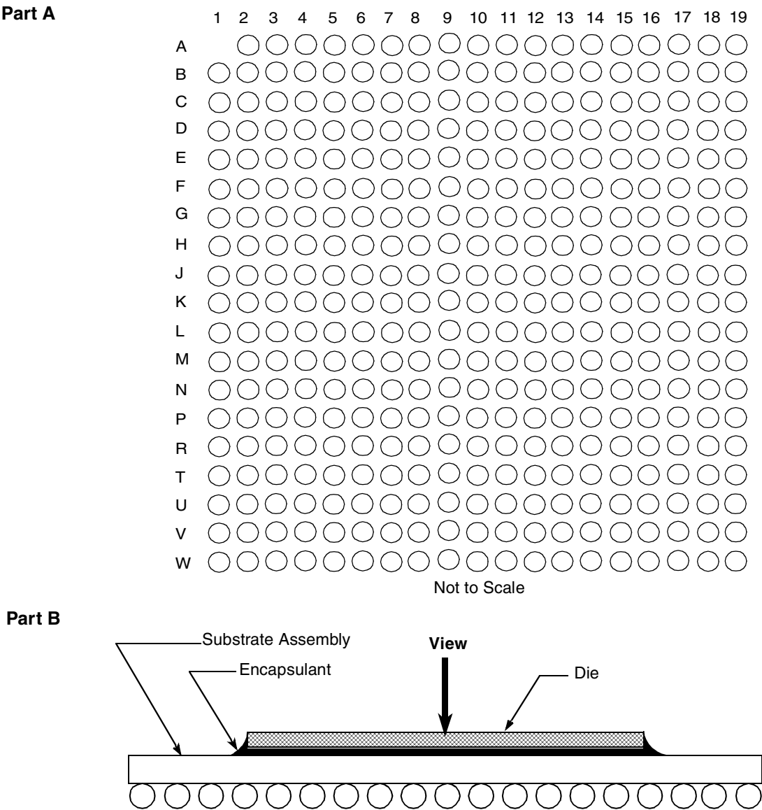
Figure 12. Pinout of the MPC7448, 360 HCTE Package as Viewed from the Top Surface
