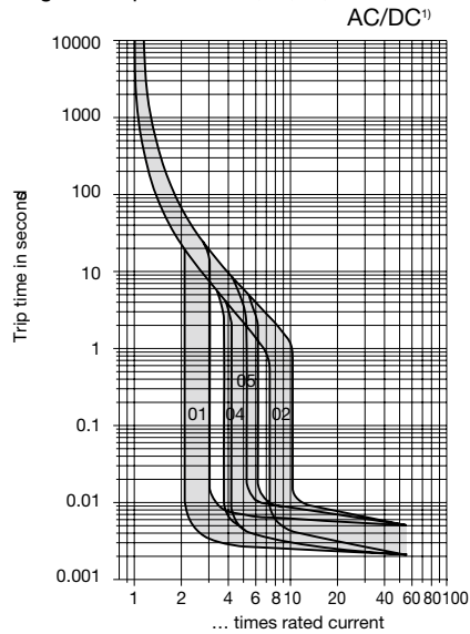
Magnetic trip curves 01,02,04,05
