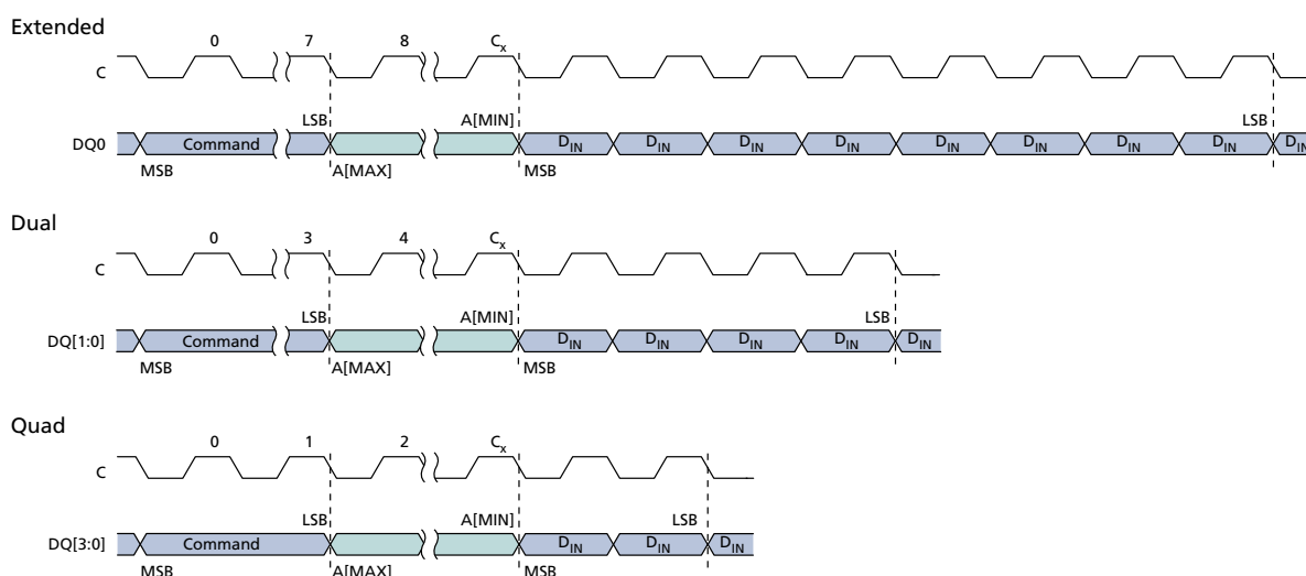
Figure 12: WRITE LOCK REGISTER Command
