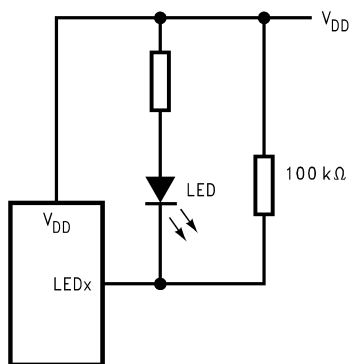
FIGURE 9. Methods to Reduce I_Q When LEDs Are Off
