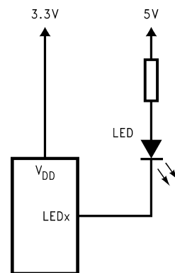
FIGURE 9. Methods to Reduce I_Q When LEDs Are Off
