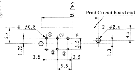
PCB mounting hole layout (Connector mounting side)
