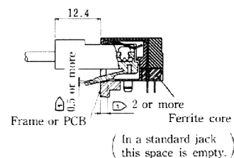
View of mating plug A-A
