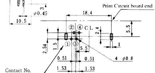
PCB mounting hole layout (Connector mounting side)
