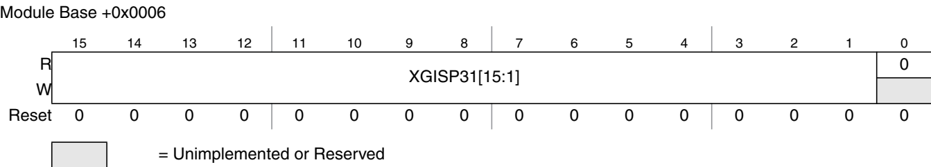
Figure 10-8. XGATE Initial Stack Pointer for Interrupt Priorities 3 to 1 (XGISP31)
