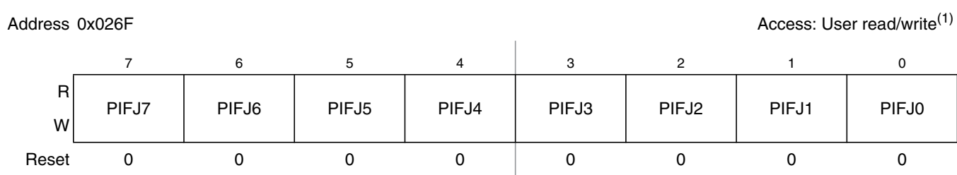
Figure 2-66. Port J Interrupt Flag Register (PIFJ)
