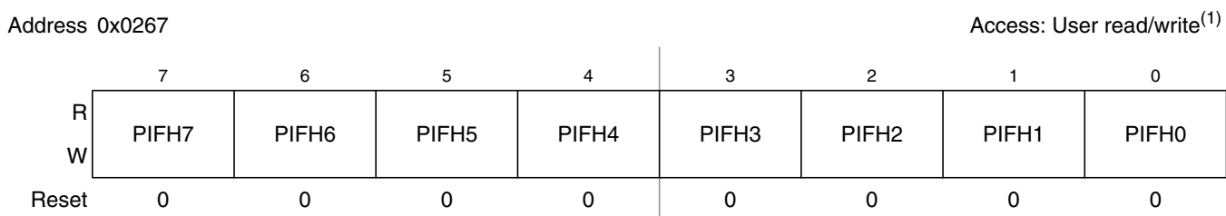
Figure 2-58. Port H Interrupt Flag Register (PIFH)
