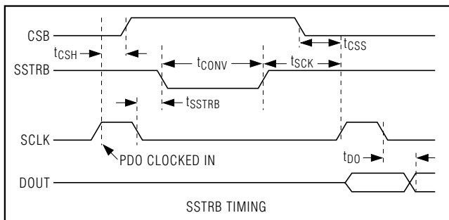
Figure 6. Detailed SSTRB Timing
