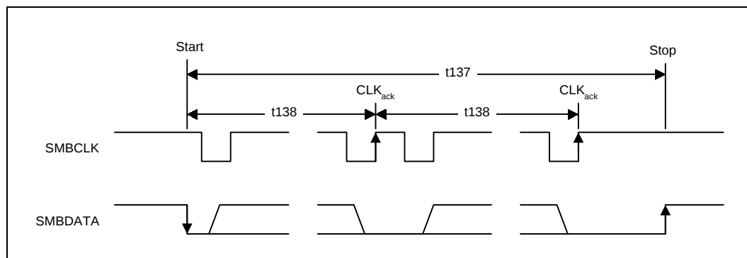
Figure 14-17. SMBus Timeout
