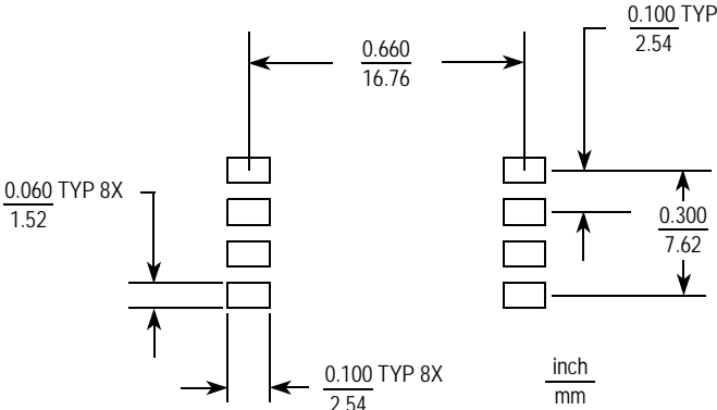
Figure 9. SOP footprint
