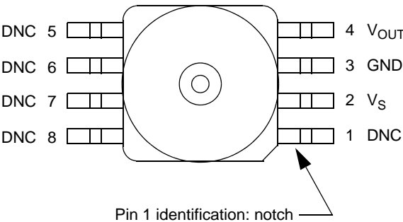
Figure 2. Device pinout (top view)
