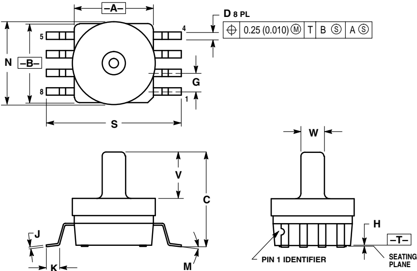
Case 98ASB17757C, small outline package
