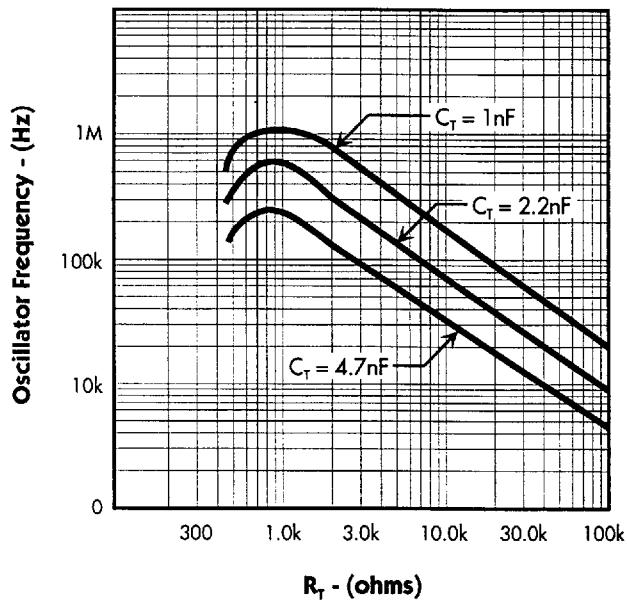
FIGURE 1. — OSCILLATOR FREQUENCY vs. TIMING RESISTOR
