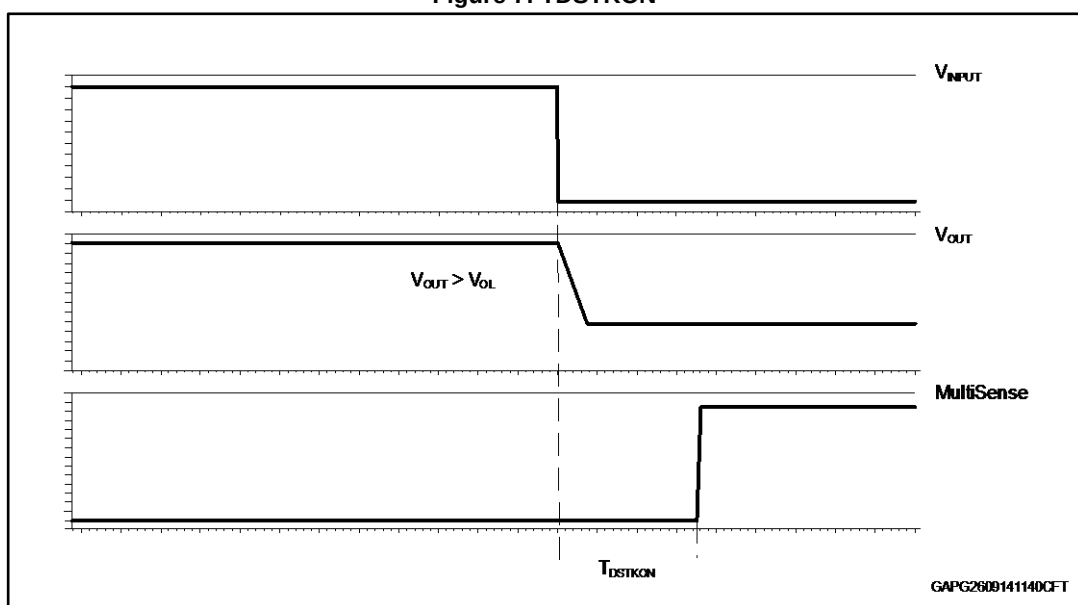
Figure 7: TDSTKON
