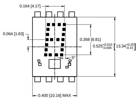
4N54
