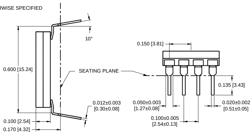
4N54
