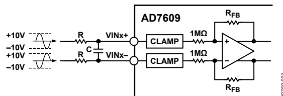
Figure 34. Input Resistance Matching on the Analog Input
