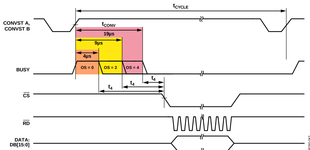
Figure 46. AD7609—No Oversampling, Oversampling \times 4 , and Oversampling \times 8 Using Read After Conversion
