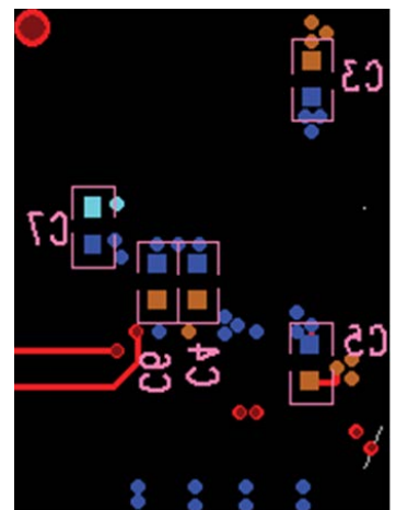
Figure 61. Bottom Layer Decoupling
