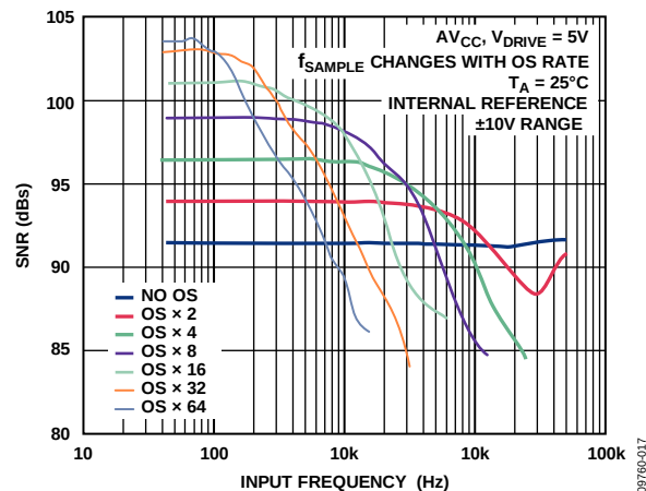
Figure 19. SNR vs. Input Frequency, \pm 10 V Range
