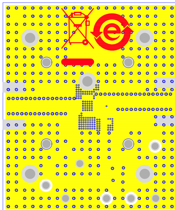
Figure 39. Evaluation Board Layout, Bottom
