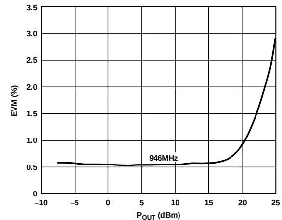
Figure 27. EVM vs. P_{OUT} , 3GPP, TM1-64, at 946 MHz
