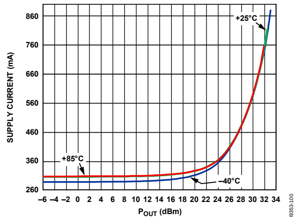
Figure 29. Supply Current vs. P_{OUT} and Temperature at 943 MHz, V_{CC} = 5\text{ V}
