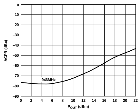
Figure 26. ACPR vs. P_{OUT} , 3GPP, TM1-64, at 946 MHz
