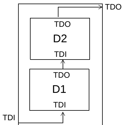
Figure 3. Scan Chain for 9-Mbit Device
