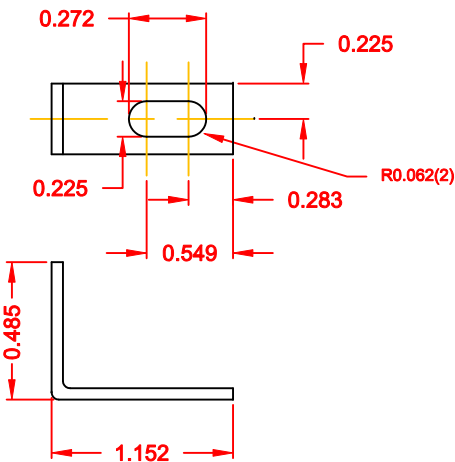
MOUNTING BRACKET
