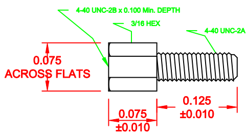
SCREW LOCK
