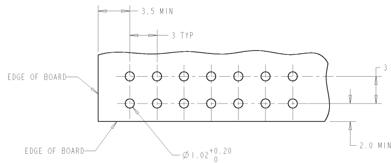
RECOMMENDED MOUNTING HOLE PATTERN SCALE 5:1
