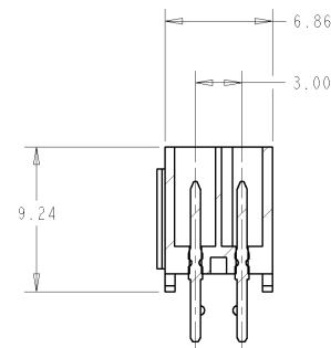
SECTION Z-Z
