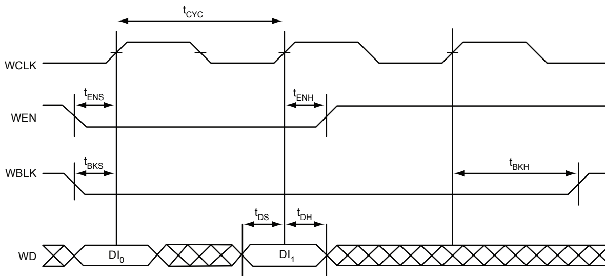
Figure 2-33 • FIFO Write
