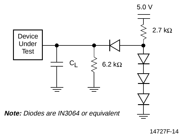
Figure 6. Test Setup
