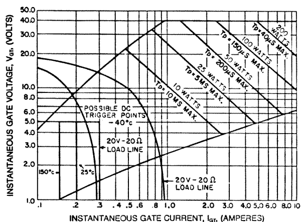
GATE CHARACTERISTICS
