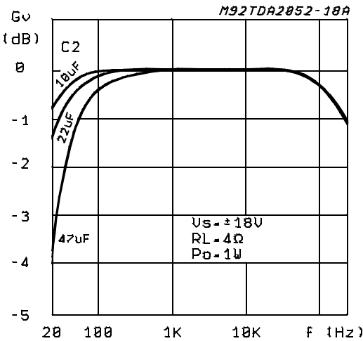
Figure 9: Bandwidth.
