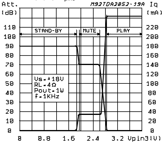
Figure 10: Output Attenuation & Quiescent Current vs. V_{pin3} .
