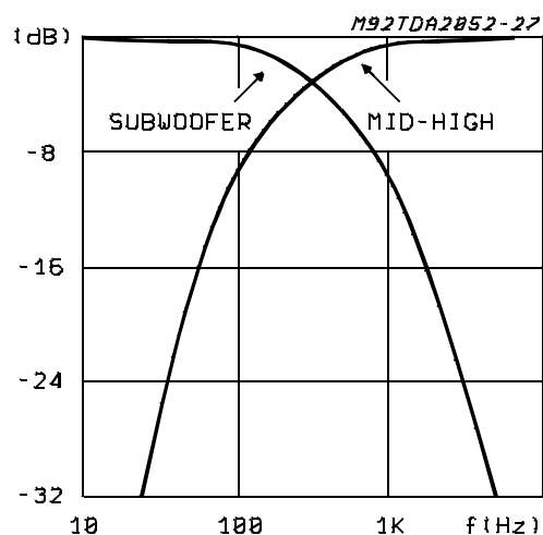
Figure 19: Frequency Response
