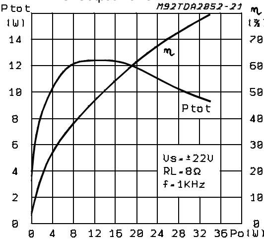
Figure 11: Total Power Dissipation & Efficiency vs. Output Power.
