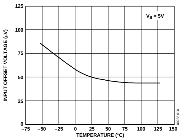
Figure 7. OP462 Input Offset Voltage vs. Temperature
