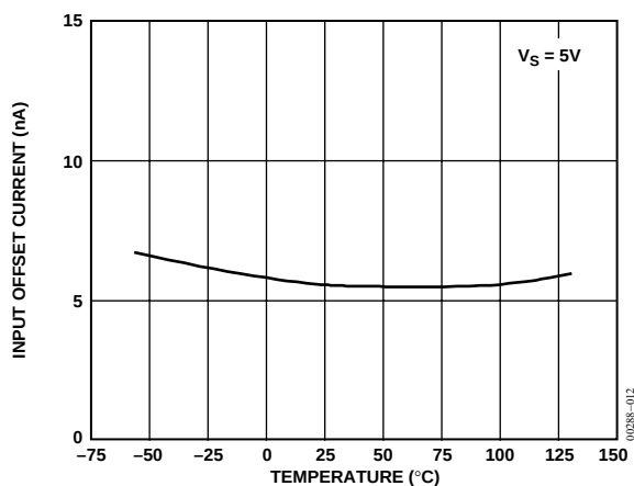
Figure 9. OP462 Input Offset Current vs. Temperature
