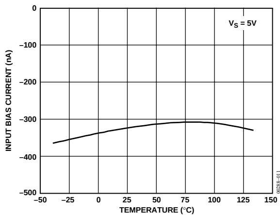
Figure 8. OP462 Input Bias Current vs. Temperature
