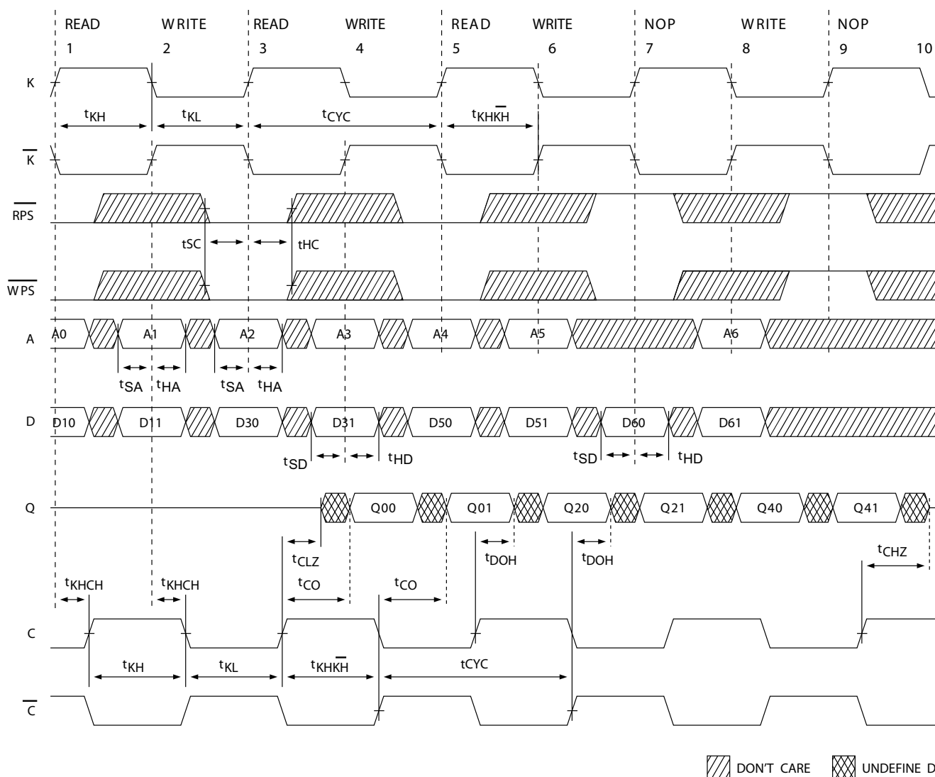
Figure 5. Switching Waveforms [29, 30, 31]
