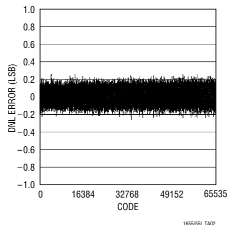
Differential Nonlinearity vs Input Code
