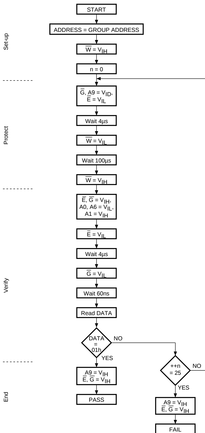
Figure 16. Programmer Equipment Group Protect Flowchart
