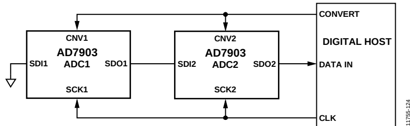
Figure 47. Chain Mode Without Busy Indicator Connection Diagram
