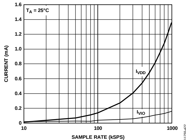
Figure 22. Operating Currents of Each ADC vs. Sample Rate
