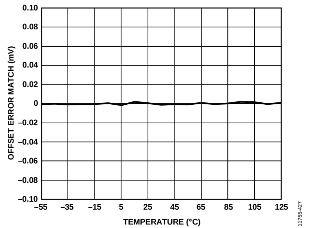
Figure 27. Offset Error Match vs. Temperature
