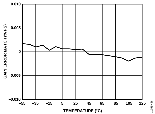
Figure 28. Gain Error Match vs. Temperature
