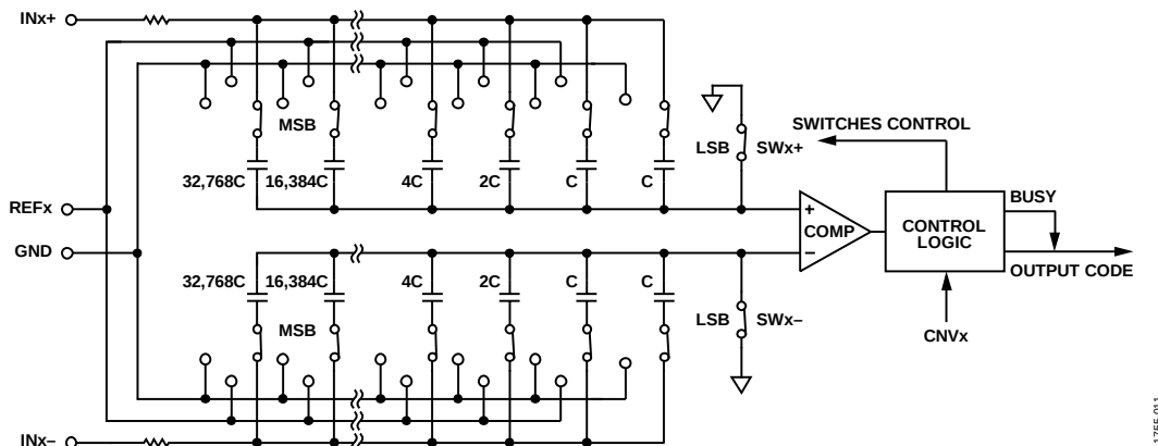
Figure 31. ADC Simplified Schematic
