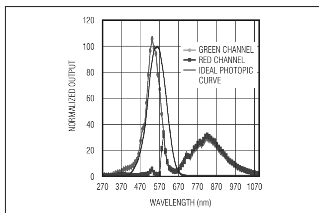
Figure 2. Green Channel and IR Channel Response at Identical Gains on a Typical MAX44004
