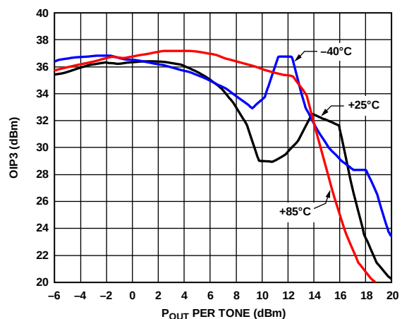
Figure 20. OIP3 vs. Output Power ( P_{OUT} ) and Temperature
