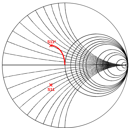
Figure 59. Smith Chart Representation of Conjugate Match
