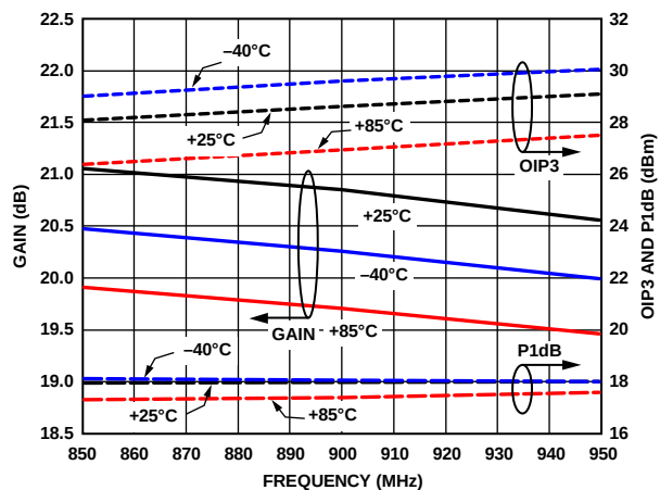
Figure 31. Gain, OIP3, and P1dB vs. Temperature
