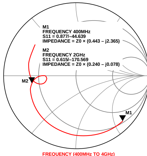
Figure 62. S11 of ADL5521 with S22 Matched at 2 GHz
