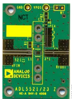
Figure 54. Evaluation Board Layout (Top View)
