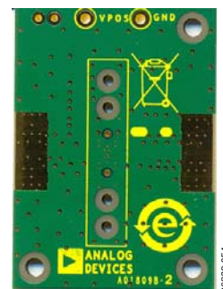
Figure 55. Evaluation Board Layout (Bottom View)
