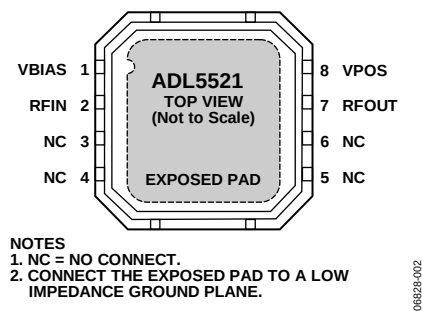
Figure 2. Pin Configuration
