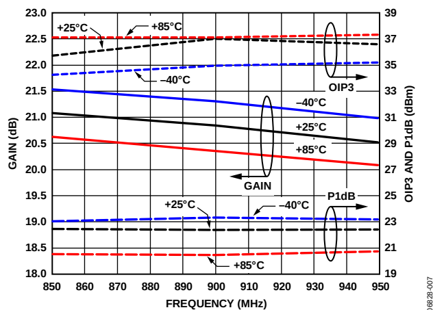
Figure 7. Gain, OIP3, and P1dB vs. Temperature
