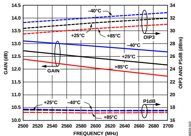
Figure 43. Gain, OIP3, and P1dB vs. Temperature
