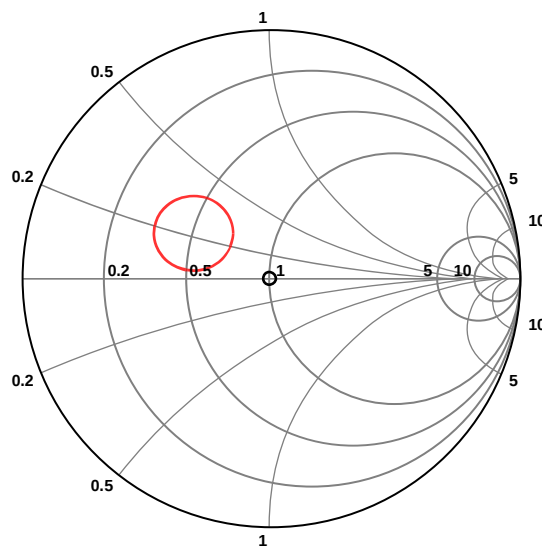
Figure 60. Area of Optimal Noise Matching for ADL5521
