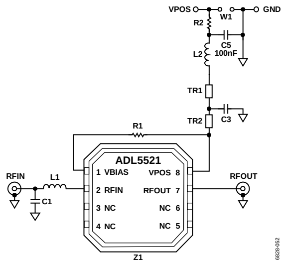
Figure 52. ADL5521 Basic Connections
