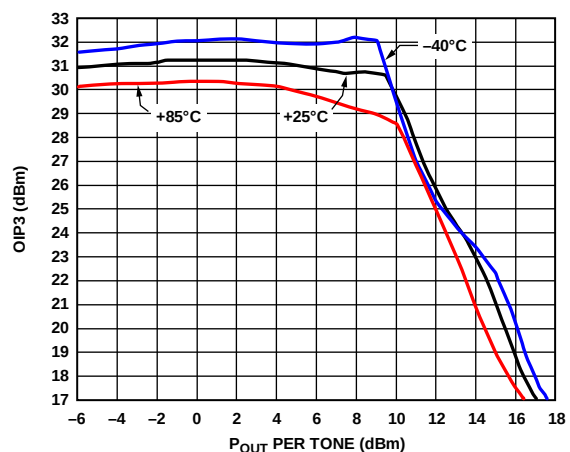
Figure 44. OIP3 vs. Output Power ( P_{OUT} ) and Temperature
