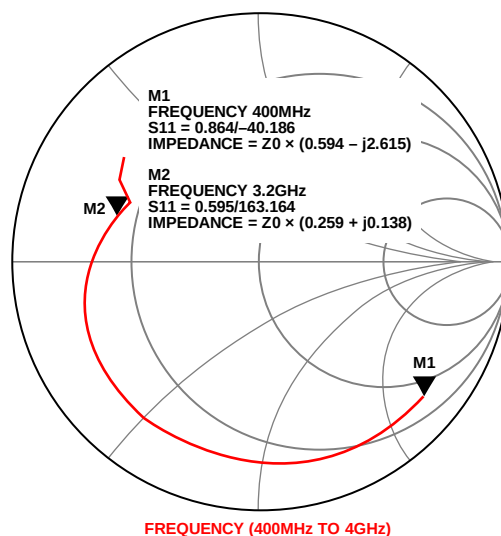
Figure 63. S11 of ADL5521 with S22 Matched at 3.2 GHz
