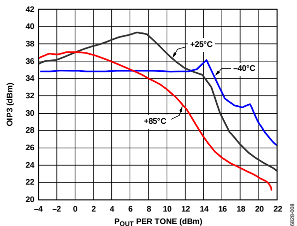
Figure 8. OIP3 vs. Output Power (P OUT ) and Temperature
