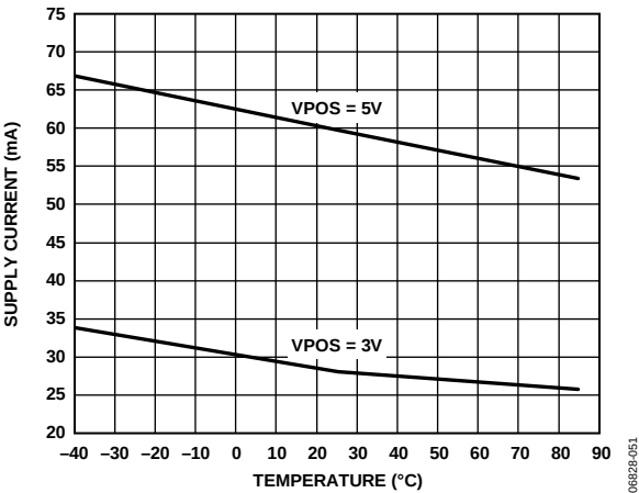
Figure 51. Supply Current vs. Temperature, 3 V and 5 V
