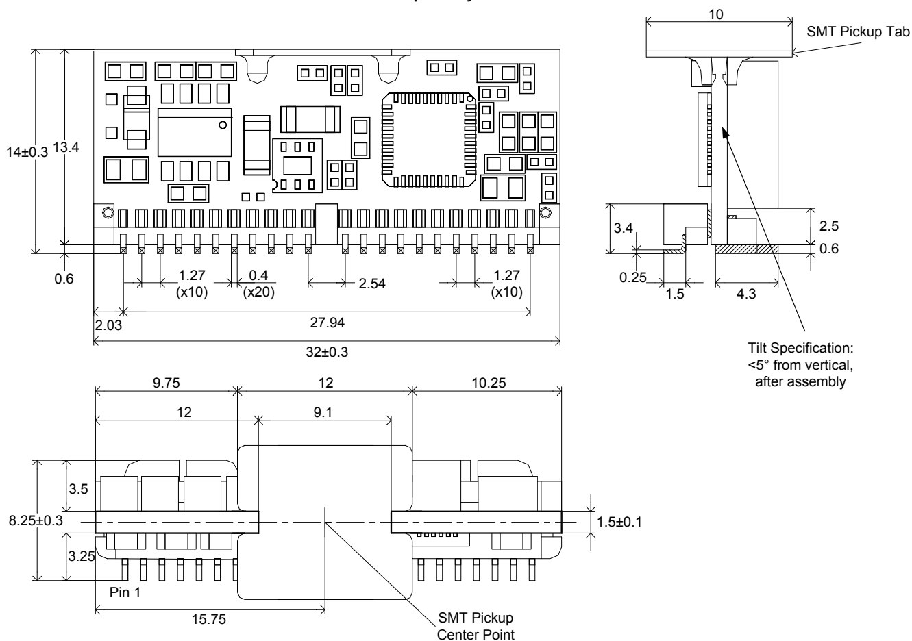
Figure 20. Mechanical Drawing
