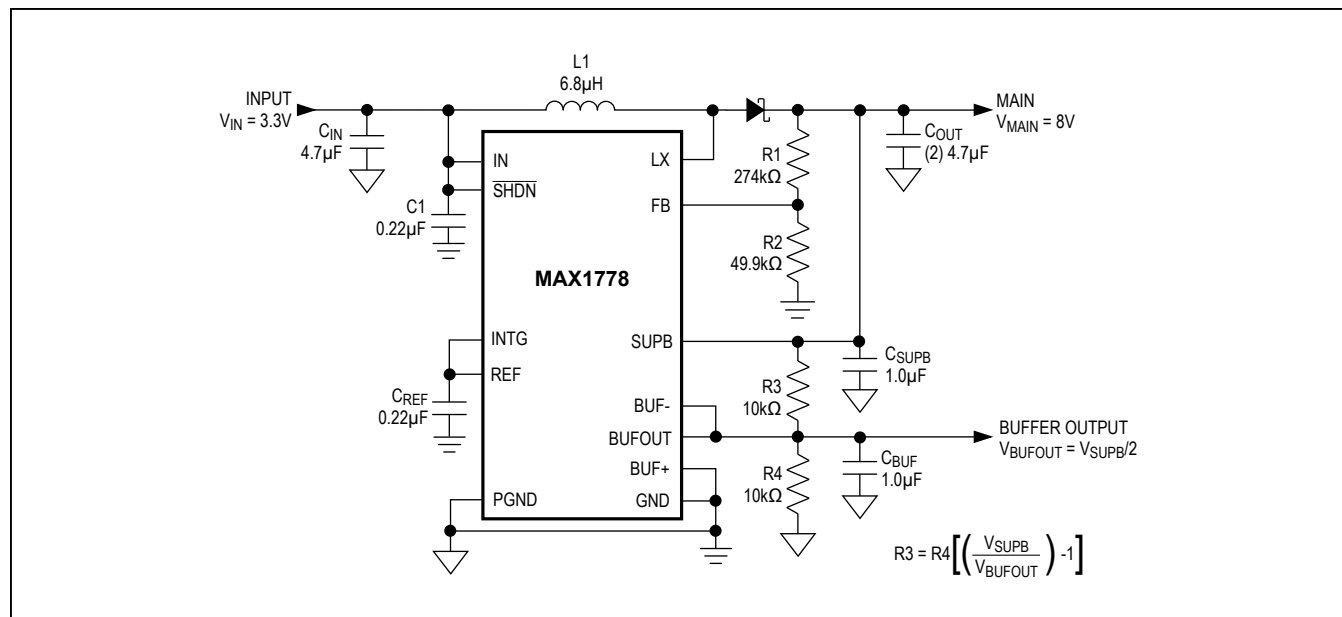
Figure 11. VCOM Buffer Soft-Start
