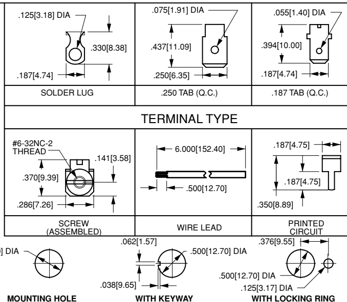
MOUNTING HOLE
