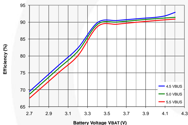
Figure 9. Efficiency vs. V_{BUS} , I_{BUSLIM}=500 mA, I_{SYS}=0
