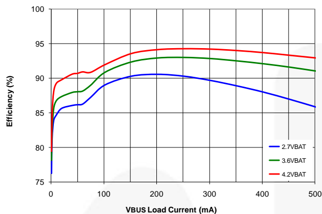
Figure 25. Efficiency vs. I_{BUS} Over V_{BAT}
