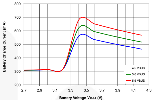
Figure 8. Battery Charge Current vs. V_{BUS} with I_{BUSLIM}=500 mA
