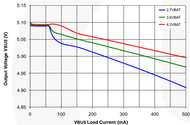
Figure 27. Regulation vs. I_{BUS} Over V_{BAT}
