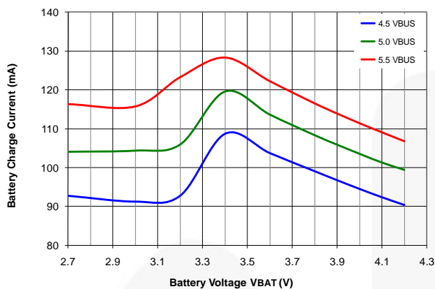
Figure 7. Battery Charge Current vs. V_{BUS} with I_{BUSLIM}=100 mA
