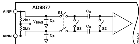
Figure 40. Differential Input Architecture
